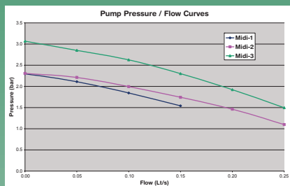
Pump Pressure / Flow Curves
