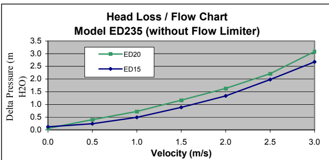
Notes - Velocity based on flow of water through the bore of copper tube table X. See Flow Table to find the actual flow rate.
